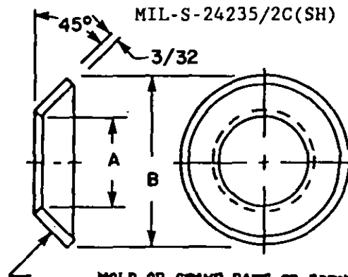
FIGURE 6. Bevel washer configuration. (06)
