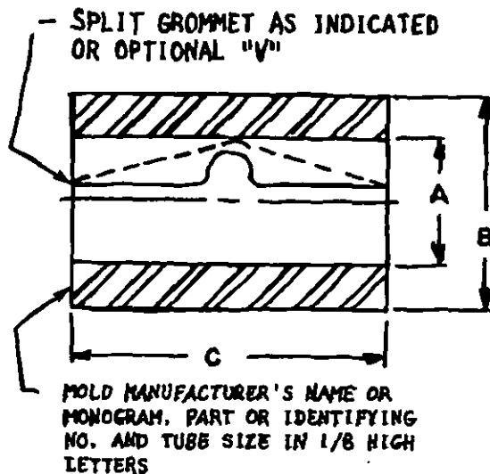
FIGURE 3. Grommet configuration for tube sizes 1, 2 and 3.
