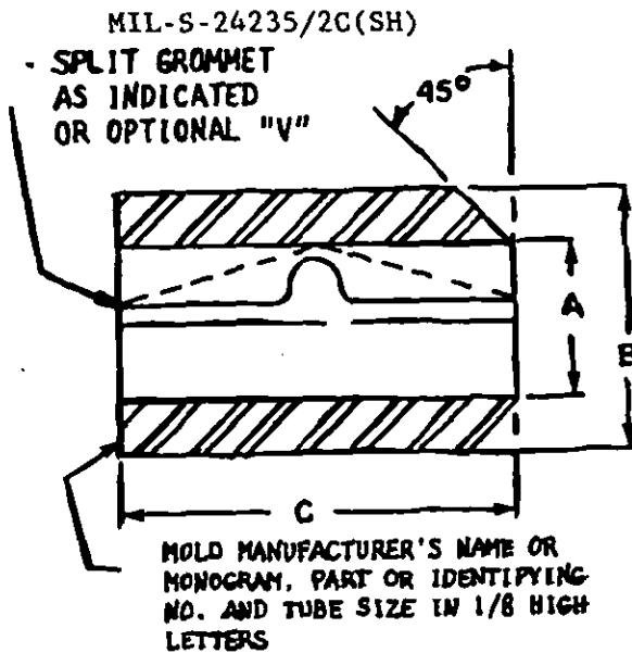
FIGURE 4. Grommet configuration for tube sizes 4 through 9.
